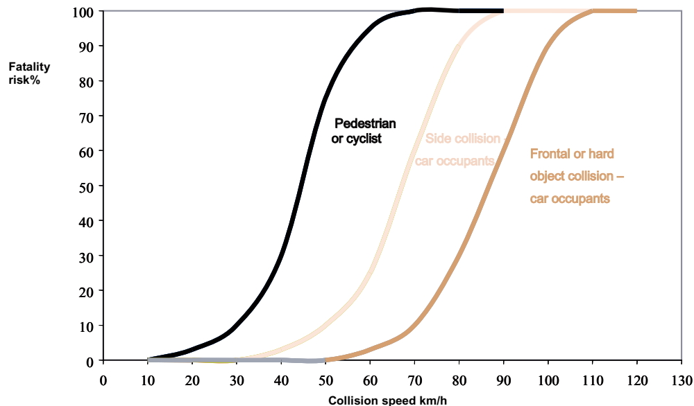
Figure 2. Fatality Risk and Collision Speed
